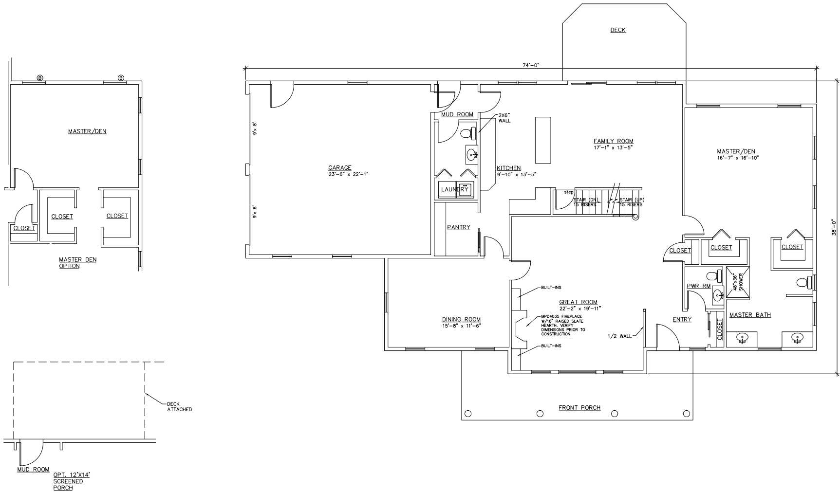
FIRST FLOOR PLAN SCALE: 1/4"=1'-0" REVISED 6/3
